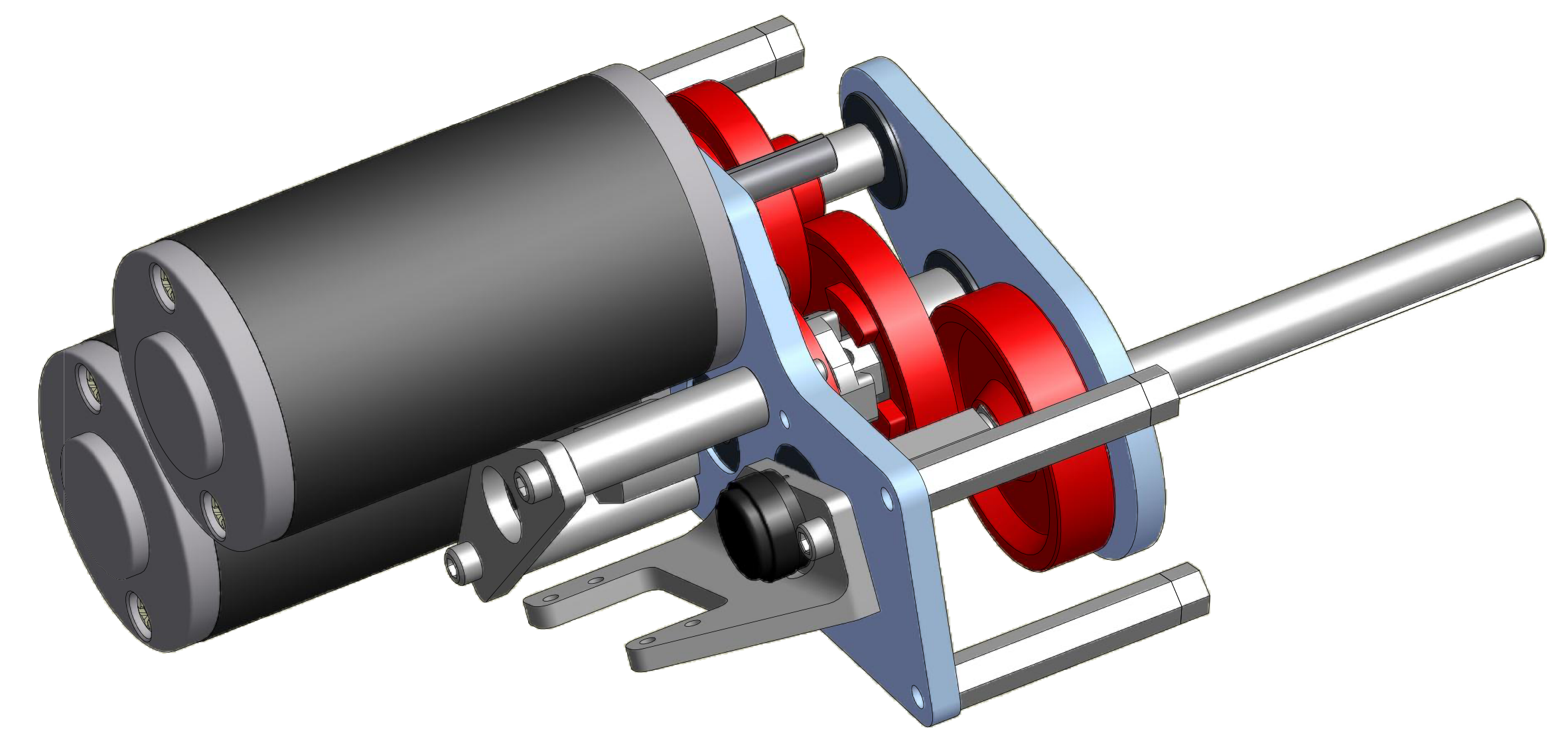
Universal Chassis SuperShifter Adapter Assembly 221 Robotics Systems LLC.
